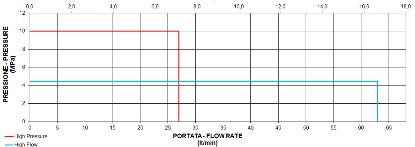
PORTATA - FLOW RATE (lt/min)
