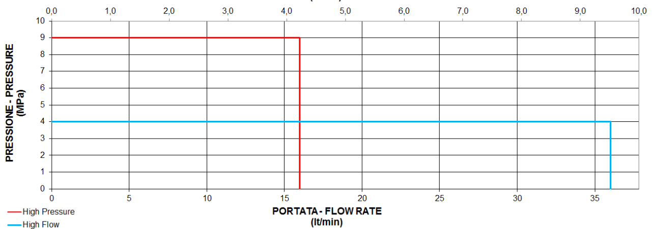
DIAGRAMMA PORTATA - PRESSIONE PRESSURE-FLOW RATE DIAGRAM
