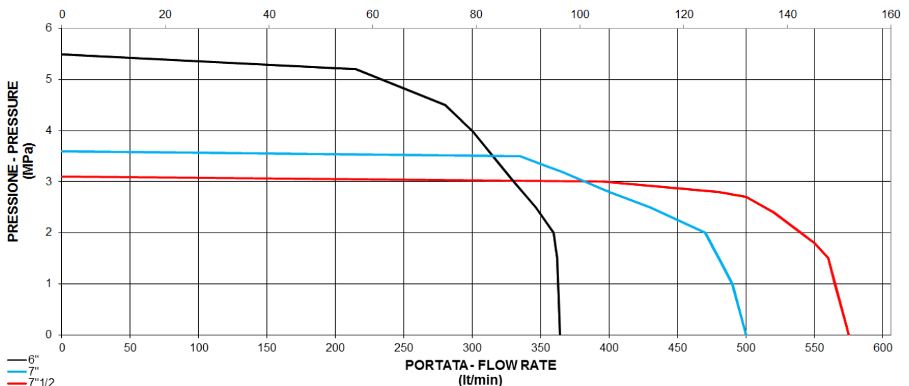
PORTATA - FLOW RATE (gpm)
