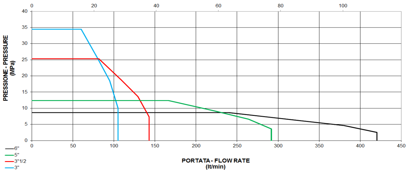
PORTATA - FLOW RATE (gpm)
